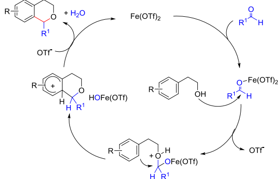
Scheme 2. Suggested mechanism for the Fe(OTf) 2 -catalyzed Oxa-Pictet-Spengler cyclization. Redraw and Make it look better.
