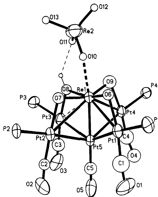
Figure 1. View of the structure of the cation [Pt 5 (CO) 5 L 4 Re(μ-O) 3 (μ-OH)(ReO 4 )] [ReO 4 ], 1 , L = P(cyclohexyl) 3 . The cyclohexyl groups are omitted for clarity. The OH proton was not directly located, and the atoms O(10)–O(13) are shown as spheres of arbitrary radius. 5
