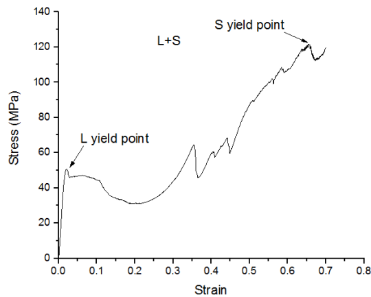
Fig. 4 Quasi-static compression stress-strain curves of an overlay of two homogeneous AMSFs (L and S)
