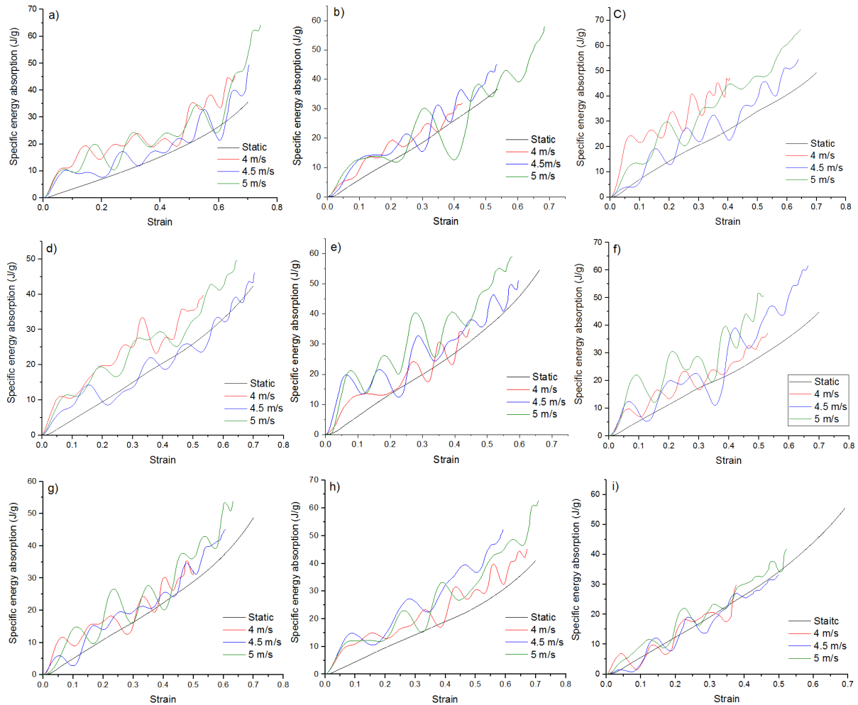
Fig. 8 Specific energy absorption as a function of strain for AMSFs: a) L, b) M, c) S, d) LM, e) MS, f) LS, g) LMS, h) MLS, i) LSM
