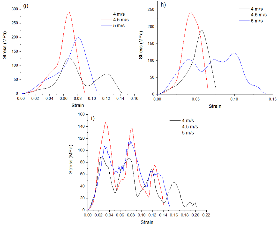
Fig. 6 Stress-strain curves for graded AMSFs under impact loading at different impact velocities: a) L, b) M, c) S, d) LM, e) MS, f) LS, g) LMS, h) MLS, and i) LSM
