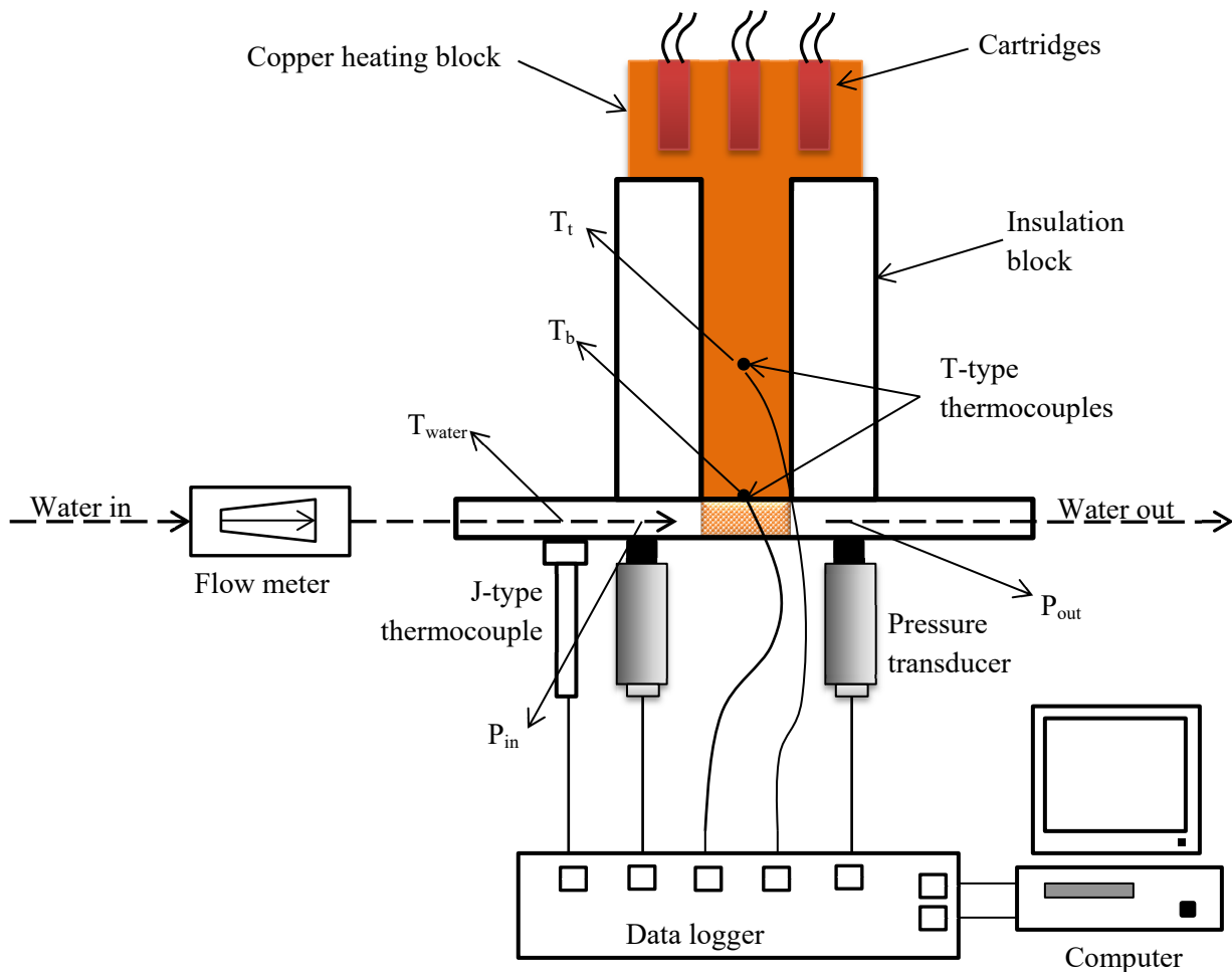
Fig. 2 Schematic diagram of the experimental apparatus for pressure drop and heat transfer coefficient measurements
