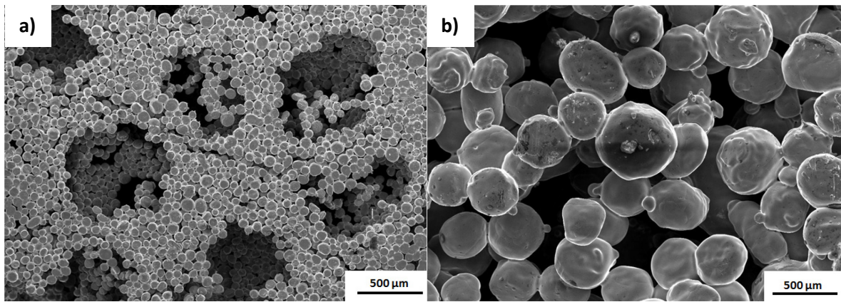
Fig. 1 SEM micrographs showing typical structures of LCS porous Cu with Cu particle sizes of (a) 75 \mu\text{m} and (b) 425 \mu\text{m}
