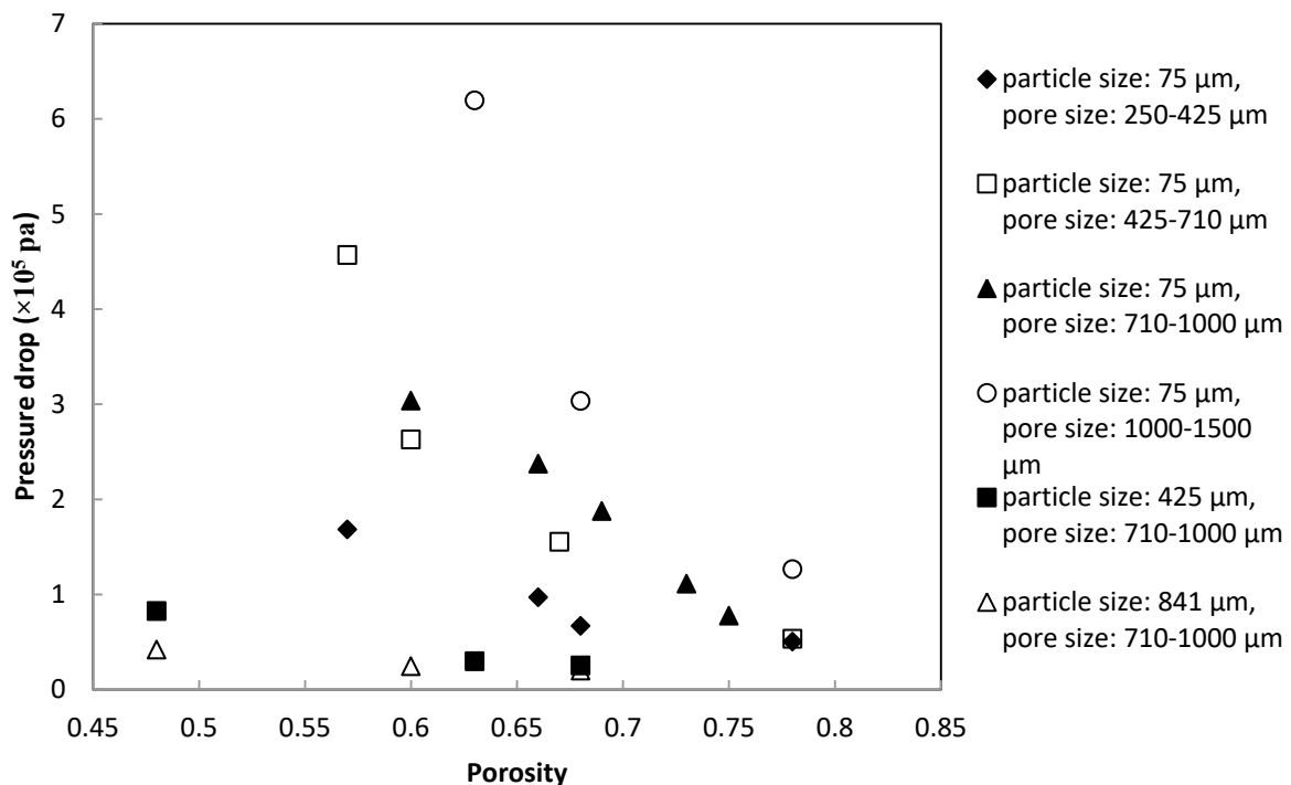
Fig. 4 Variations of pressure drop as a function of porosity, pore size and Cu particle size at a flow rate of 2.0 L/min
