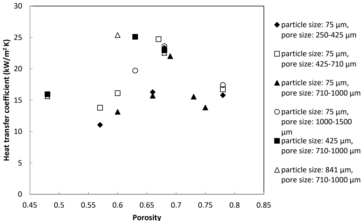
Fig. 3 Variations of heat transfer coefficient as a function of porosity, pore size and Cu particle size at a flow rate of 2.0 \text{ L/min}
