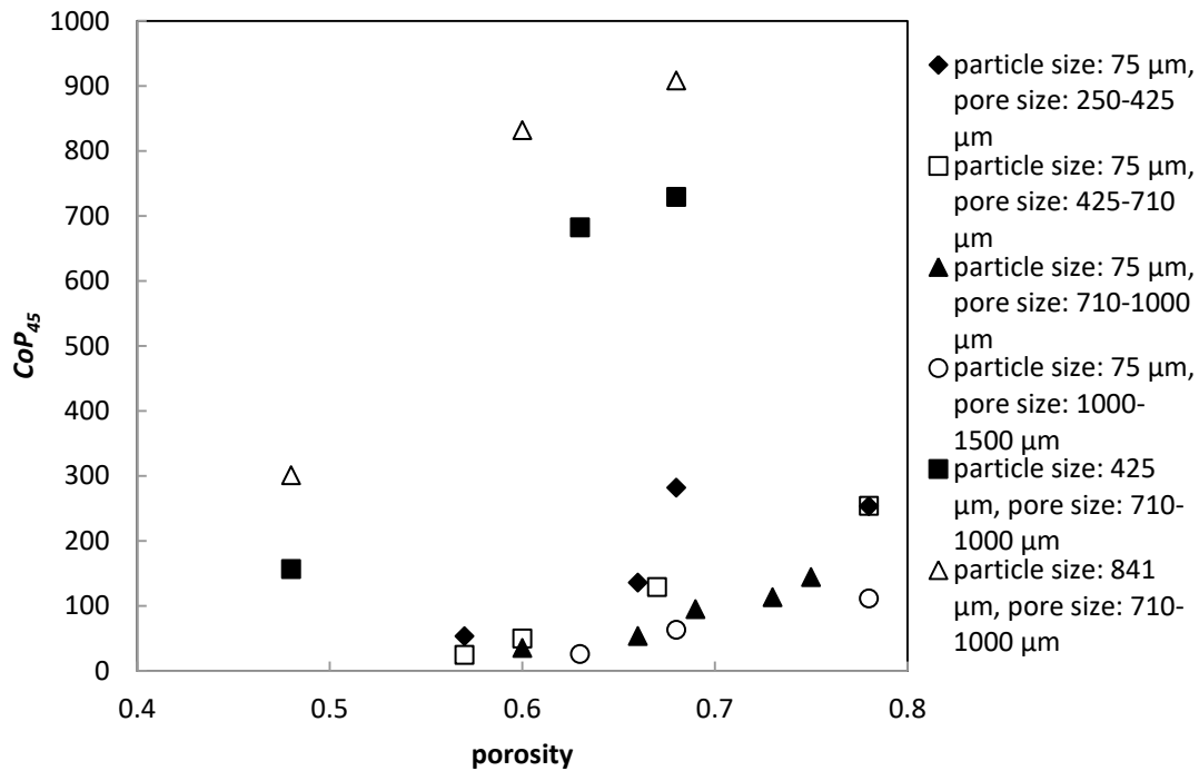
Fig. 5 Variations of coefficient of performance ( CoP_{45} ) as a function of porosity, pore size and Cu particle size at a flow rate of 2.0 L/min
