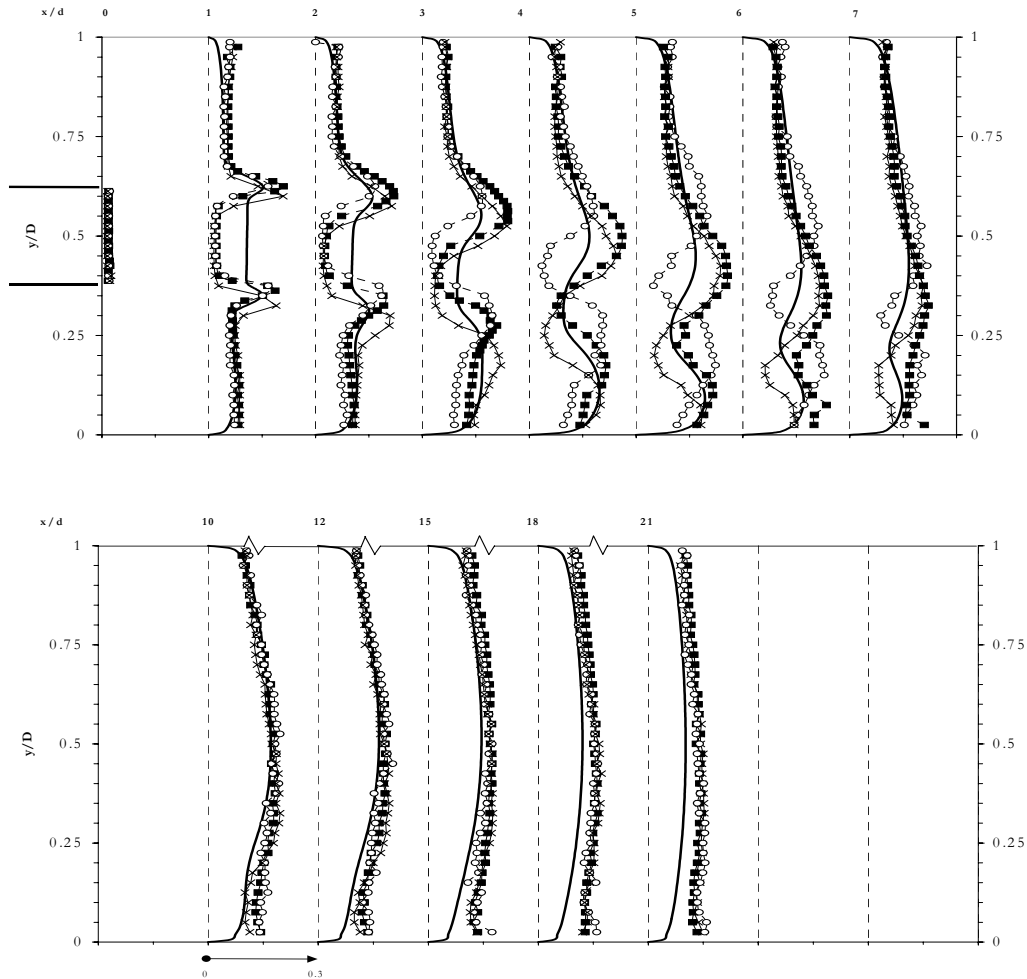
Figure 6: RMS axial turbulence intensity profiles ( u'/U_B ) for three XY-planes \times z=15 mm \blacksquare z=40 mm \circ z=65 mm — k-\epsilon model
