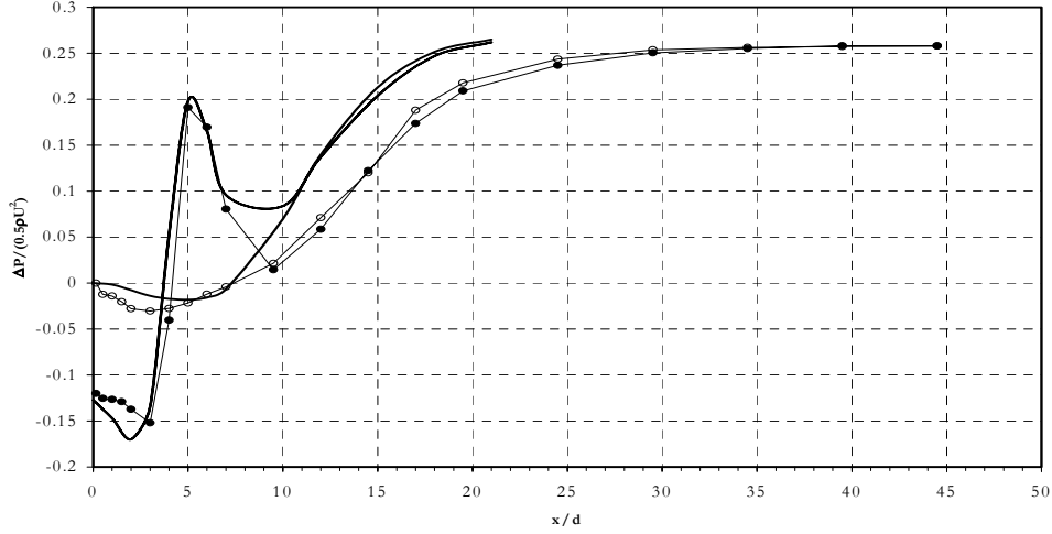
Figure 2: Wall pressure variation for the XY-centreplane ( ● lower side ○ upper side — k- \epsilon model )
