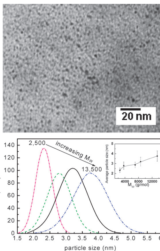
Fig. 1 TEM image of the Co NPs synthesized in the presence of the PMAA-DDT polymer (molecular weight M_w = 8610 \text{ g mol}^{-1} ) (upper panel); size distribution histograms of the Co NPs synthesized in the presence of PMAA-DDT polymers with different molecular weights at a concentration of 0.12 mM (bottom panel); the inset shows the average particle size as a function of the polymer molecular weight.
