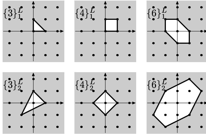
FIGURE 3. The lattice-regular polygons with edges of unit length.
