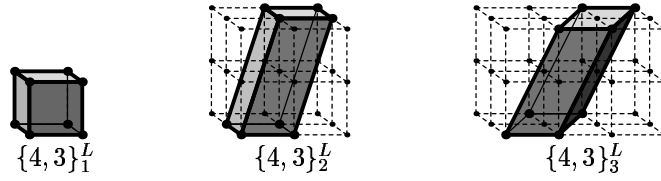
FIGURE 5. Three-dimensional elementary lattice-regular convex lattice cubes.
