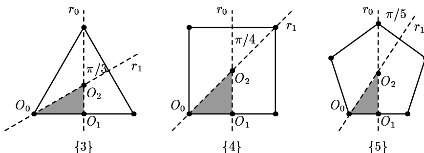
FIGURE 1. Basic reflections and Schläfli symbols for some regular polygons.
