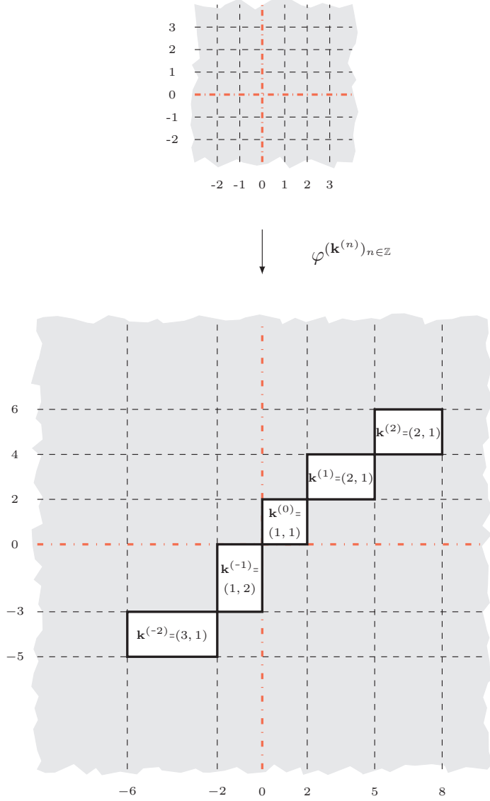
FIGURE 1. An example of sequence (\mathbf{k}^{(n)})_{n \in \mathbb{Z}} of 2-dimensional vectors with entries in the naturals and the function \varphi(\mathbf{k}^{(n)})_{n \in \mathbb{Z}} that define a rigid partition of \mathbb{Z}^2 . The sequence (\mathbf{k}^{(n)})_{n \in \mathbb{Z}} represents the sizes of the rectangles of the rigid partition.
