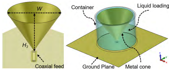
FIGURE 4. A metal cone-shaped monopole antenna is loaded by using the proposed liquid. the dimensions of the metal cone are: H_3 (height of the cone) = 39.6 mm, G (length and width of the ground plane) = 100 mm, and W (diameter of the cone) = 49 mm. The overall dimension of the antenna is still 100 \times 100 \times 41 \text{ mm}^3 .
