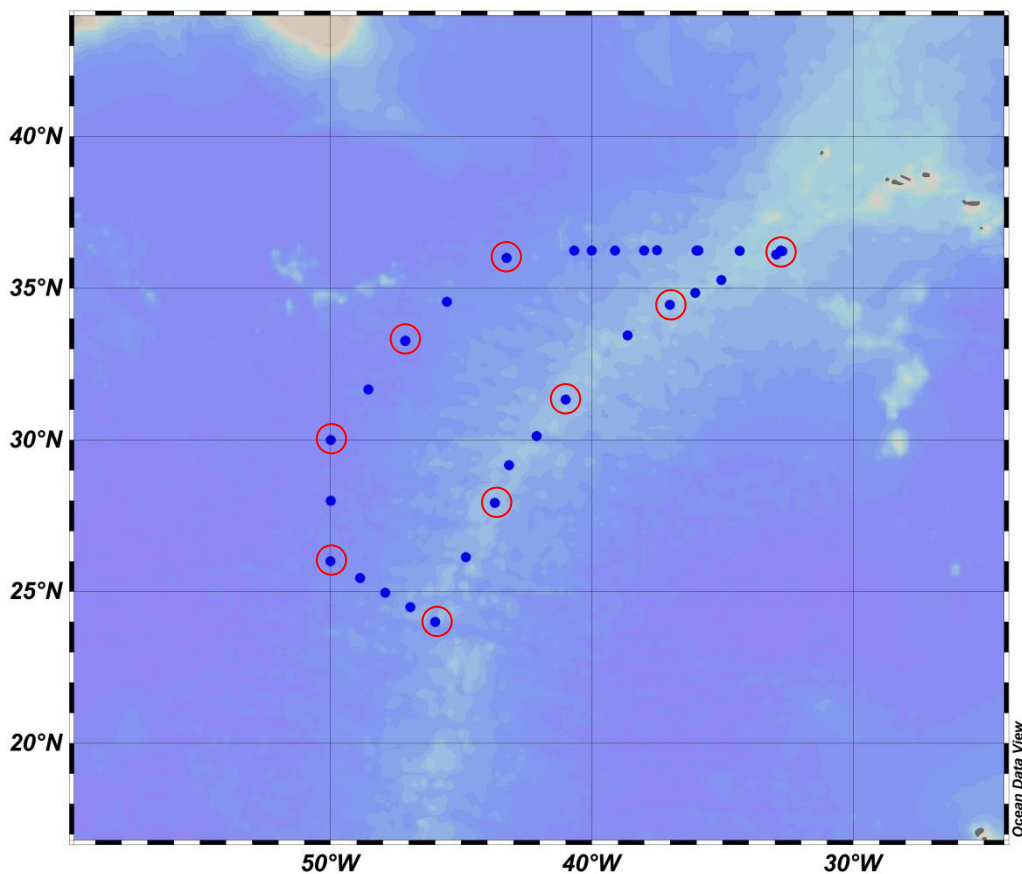
Location of stations sampled: blue dots = CTD sampling; red circles = stations with SAPs and zooplankton nets.
