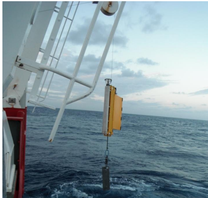
Figure 4 – Deployment of the sub-surface weight, line and wirewalker
