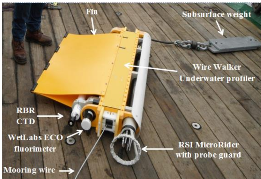
Figure 2 - Wirewalker underwater profiling system key features
