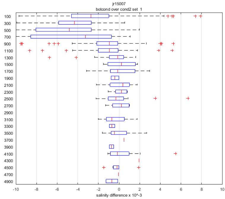
Figure 10: Series of box plots calculated in 200m bins post calibrations for the preferred sensor (secondary). The red lines indicate the median, the blue boxes the interquartile range and the black lines the full range. Data points more than 1.5 times the interquartile range away from q1 or q3 are excluded.
