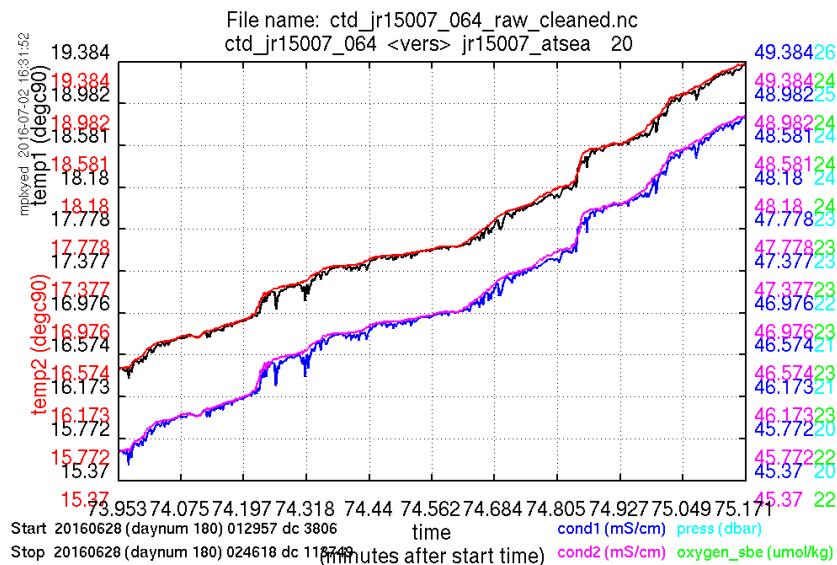
Figure 2: Temperature and conductivity time-series from CTD 64 showing the periods of mismatch still existing after changing the primary sensors
