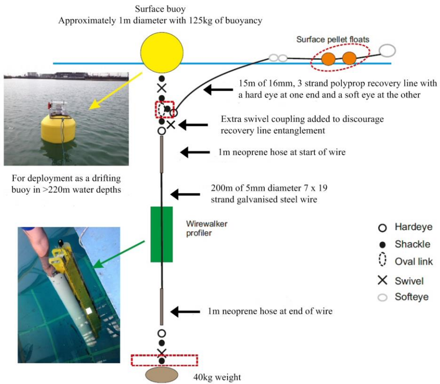
Figure 1 - Basic mooring layout of the wirewalker underwater profiling system
