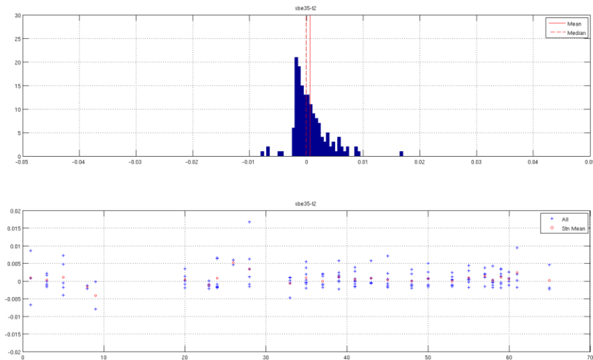
Figure 4: SBE35 minus the secondary temperature sensor after calibration for depths greater than 2000db. (a) Histogram of temperature difference with the mean and median marked with red lines. (b) Temperature difference by station, with the station mean marked in red.
