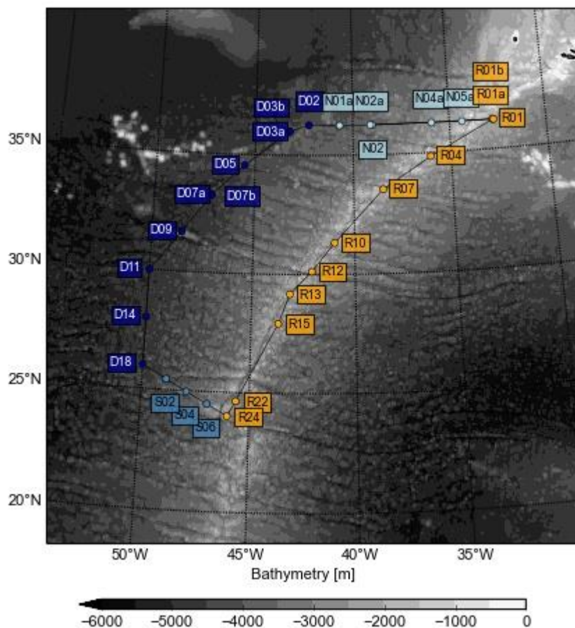
Figure 1: Bathymetry and VMP6000 stations. VMP2000 profiles were done on stations R01 and D03. (JR15-007)
