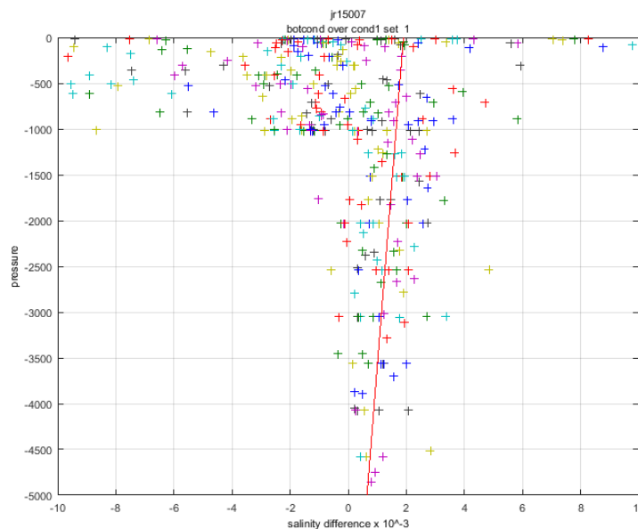
Figure 7: Vertical profile of the difference between the conductivity given from bottle samples and the first primary sensor. The conductivity difference has been scaled to an equivalent salinity difference. The linear fit used for calibration is show in red.
