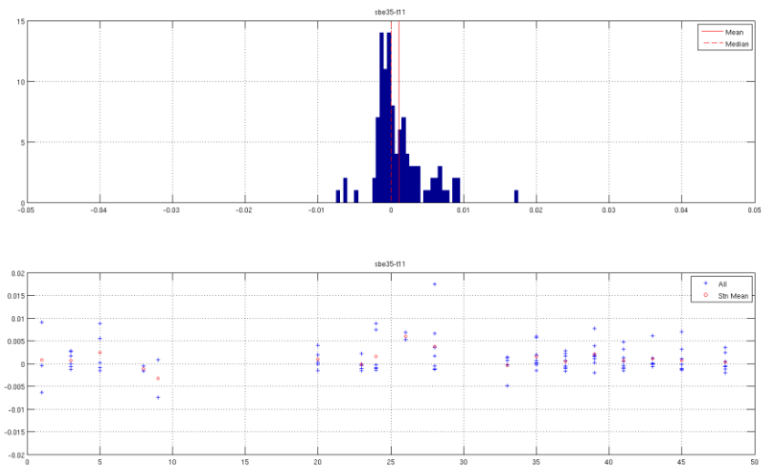
Figure 2: SBE35 minus the first primary temperature sensor after calibration for depths greater than 2000dB. (a) Histogram of temperature difference with the mean and median marked with red lines. (b) Temperature difference by station, with the station mean marked in red.
