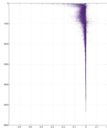
Figure 1: Vertical profiles of (a) the difference between the sbe35 recorded temperature and the temperature from the secondary temperature sensor ( ^{\circ}\text{C} ) and (b) the vertical temperature gradient ( ^{\circ}\text{Cm}^{-1} ) calculated from the 2dB downcast temperature.
