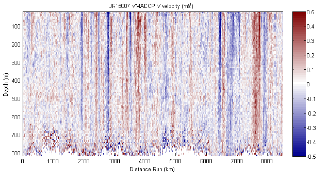
Figure 10: VMADCP V velocity ( \text{m s}^{-1} ) recorded during JR15007
