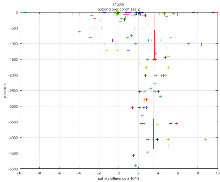
Figure 8: Vertical profile of the difference between the conductivity given from bottle samples and the first primary sensor. The conductivity difference has been scaled to an equivalent salinity difference. The linear fit used for calibration is show in red.
