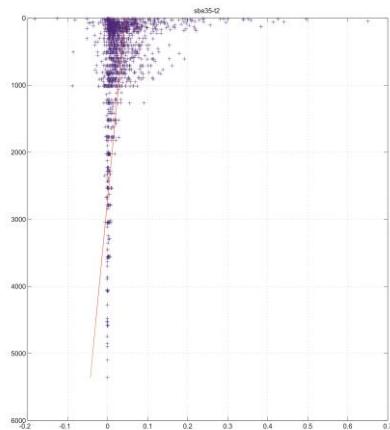
Figure 1: Vertical profiles of (a) the difference between the sbe35 recorded temperature and the temperature from the secondary temperature sensor ( ^{\circ}\text{C} ) and (b) the vertical temperature gradient ( ^{\circ}\text{Cm}^{-1} ) calculated from the 2dB downcast temperature.
