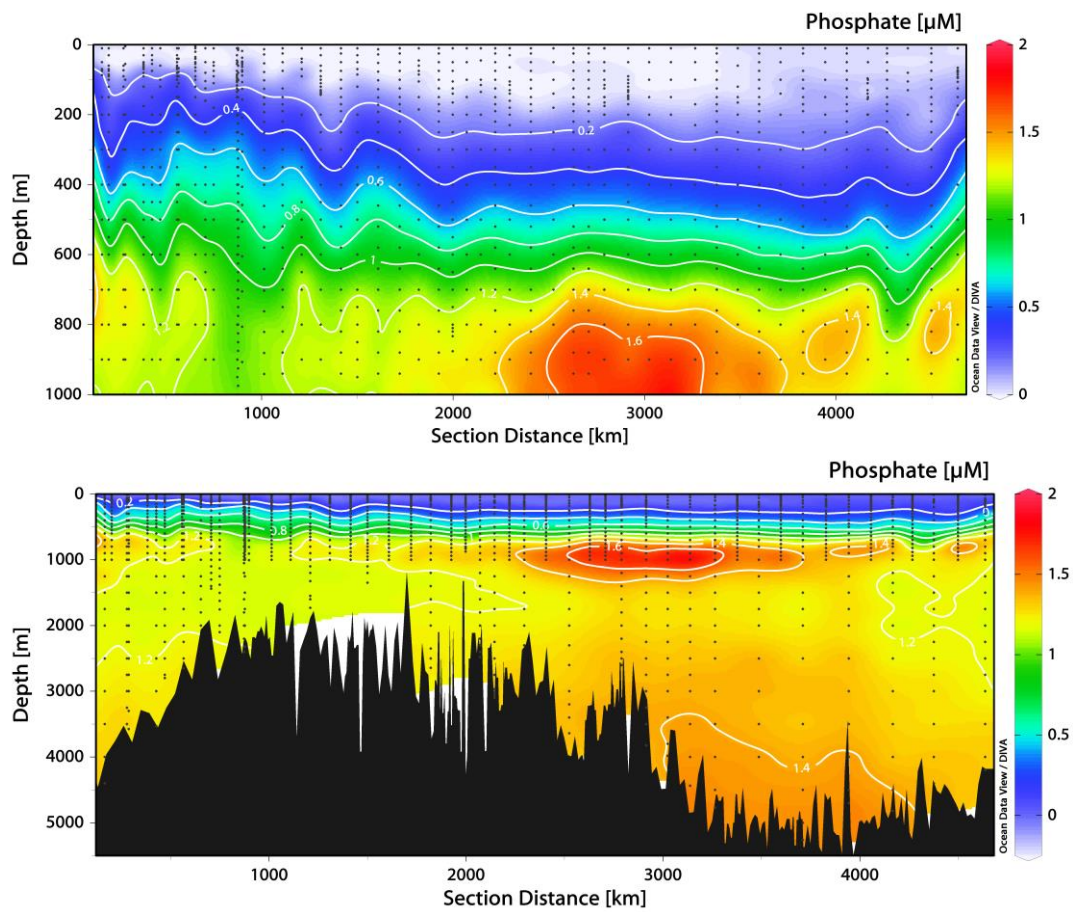
Figure 5. Phosphate concentrations ( \mu\text{mol L}^{-1} ) across the Ridgemix transect (a. 1000m, b. full water column).
