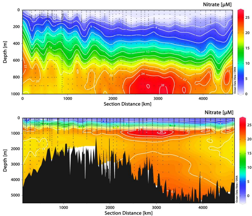
Figure 2. Nitrate concentrations ( \mu\text{mol L}^{-1} ) across the Ridgemix transect (a. 1000m, b. full water column).
