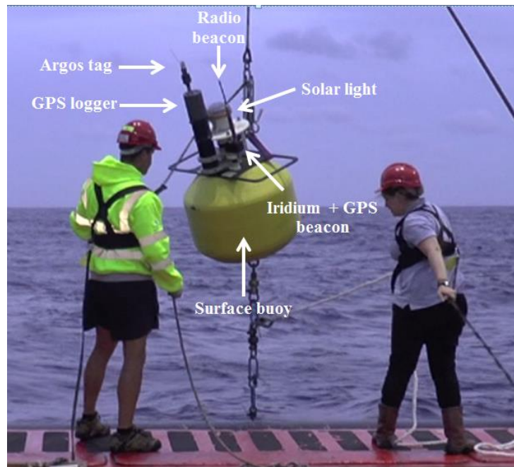
Figure 3 - Wirewalker mooring surface buoy key features
