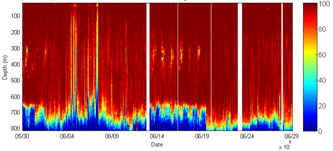
Figure JR15007 VMADCP Percentage Good
