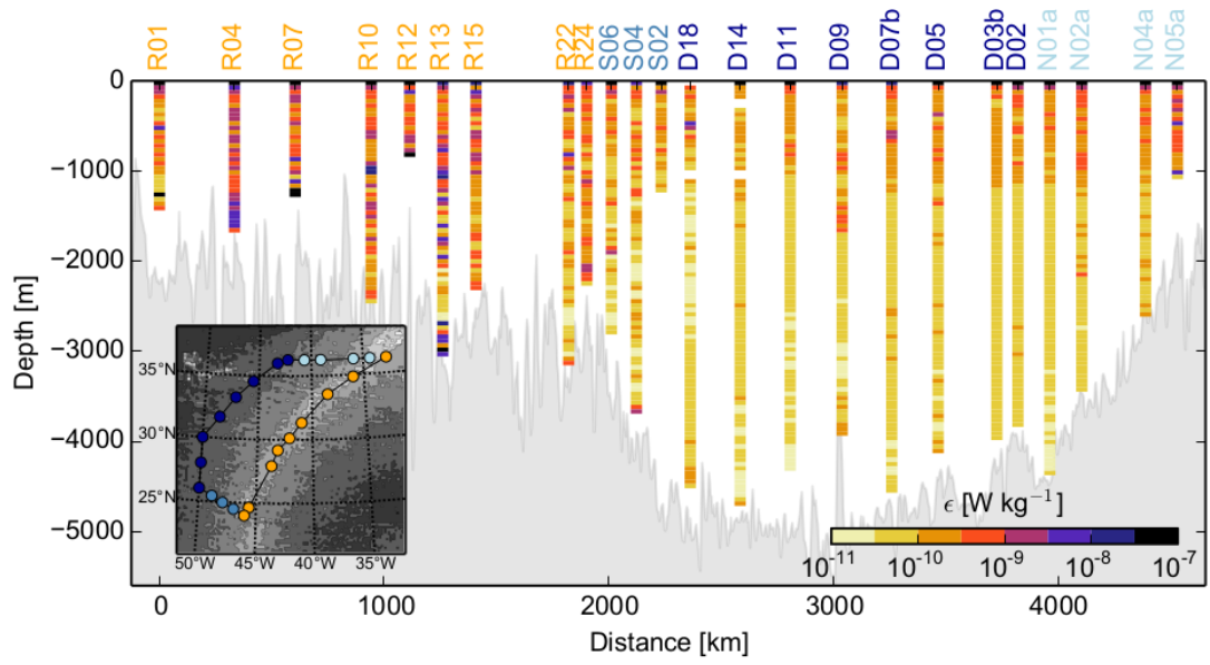
Figure 2: Kinetic energy dissipation from VMP6000 measurements. Stations in the top x-axis are reported in Figure 1.
