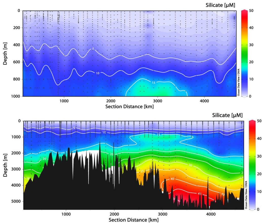
Figure 4. Silicate concentrations ( \mu\text{mol L}^{-1} ) across the Ridgeway transect (a. 1000m, b. full water column).
