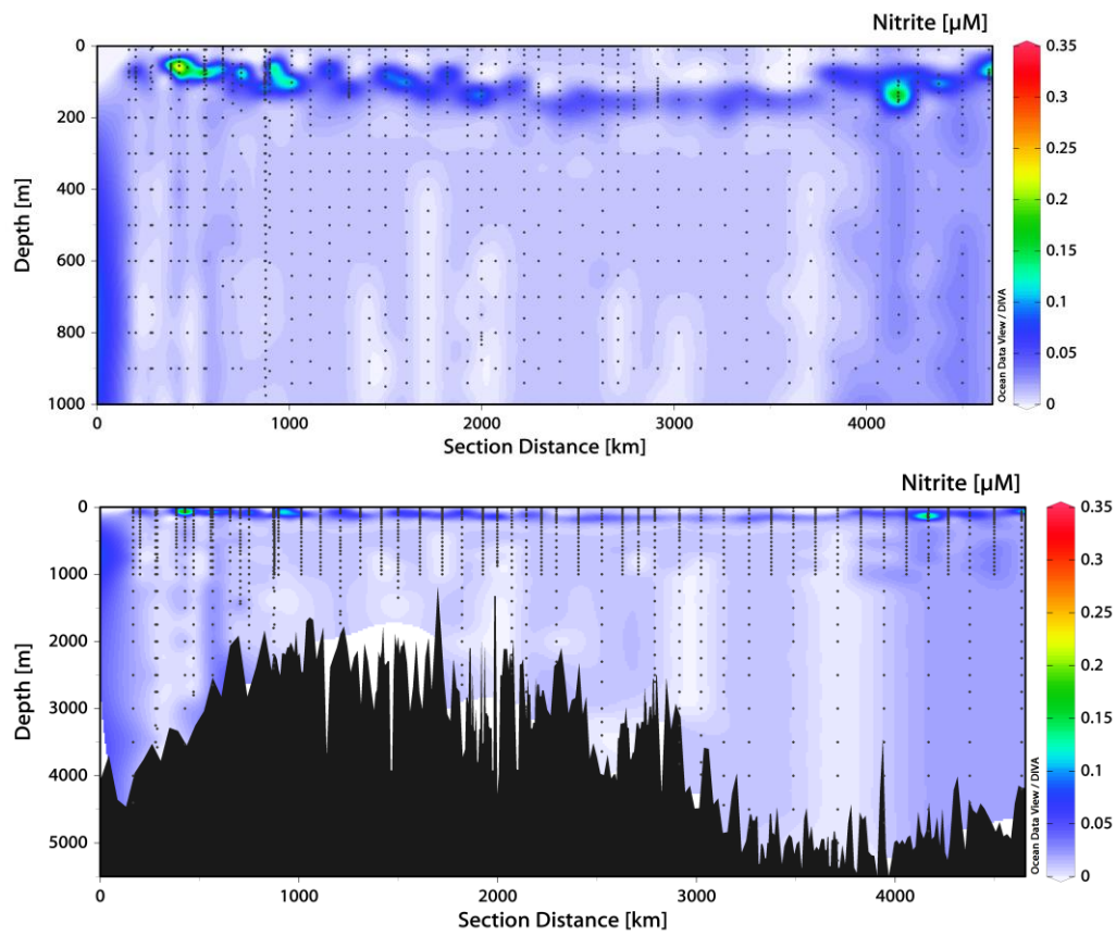
Figure 3. Nitrite concentrations ( \mu\text{mol L}^{-1} ) across the Ridgemix transect (a. 1000m, b. full water column).
