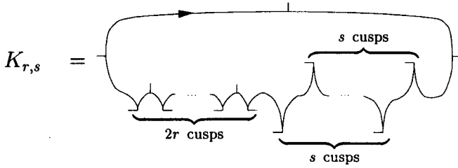
Fig. 4. Canonical curves 2
