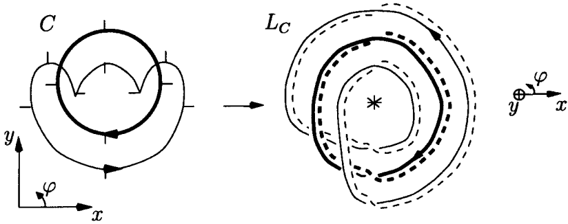
Fig. 1. Legendrian lifting
