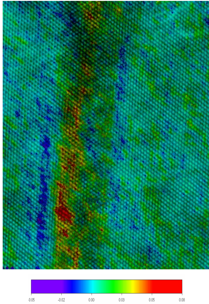
Figure 3. InGaAsN/GaAs quantum well heterostructure
