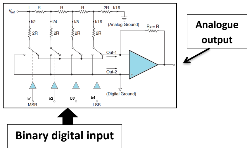
Figure 11b A binary Digital-to-Analogue Converter (bDAC) for the second Solar-Digital Revolution
