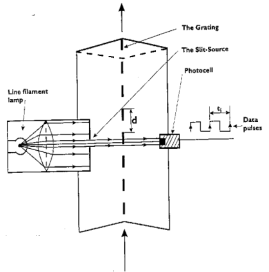
The principle of the Slit-source, Grating and Photocell method (SGP)
