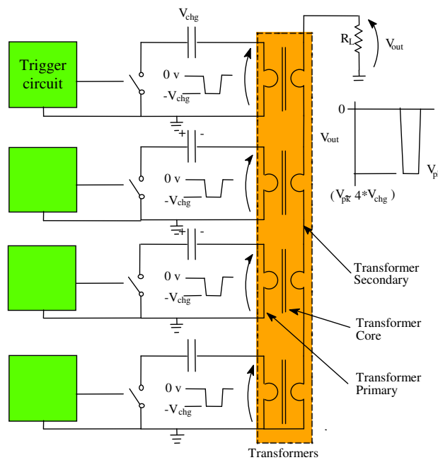
Inductive adder concept: simplified schematic. (Ed Cook)
