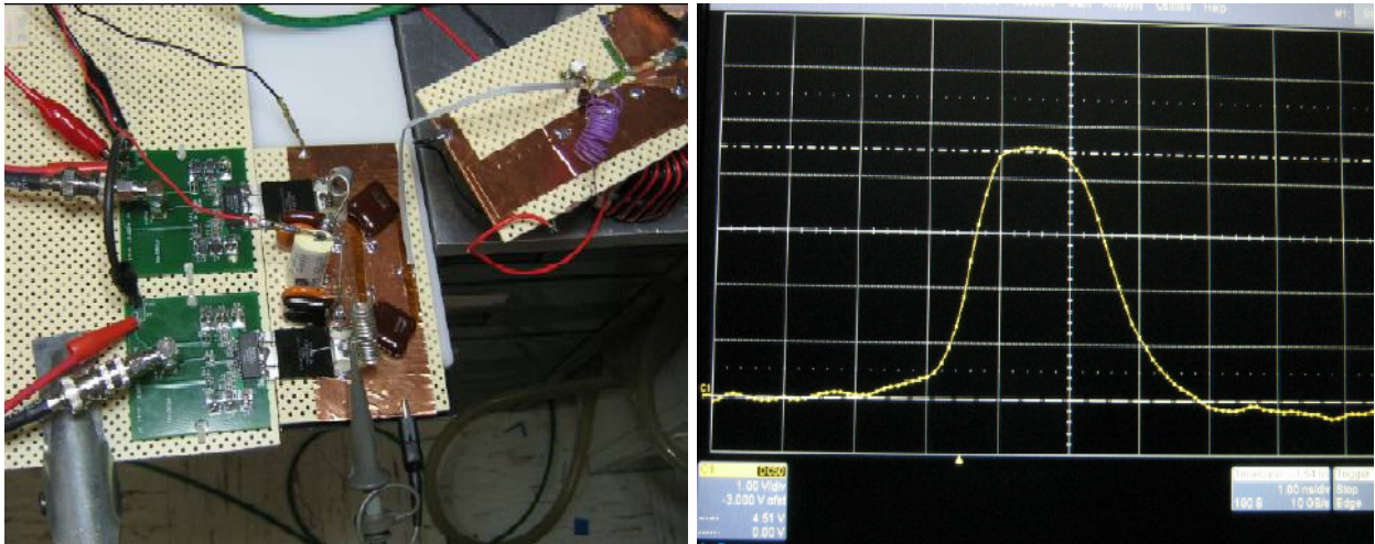
Tests of DSRD fast pulser. Output voltage 2.7 kV; horizontal scale 1 ns/division. (Anatoly Krasnykh)
